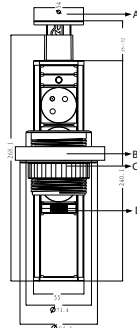
Fig.2 Technical dimensions
