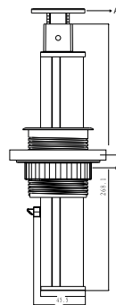
Fig.1 Technical dimensions
