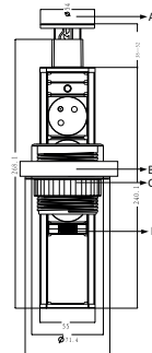
Fig.2 Dimensions techniques
